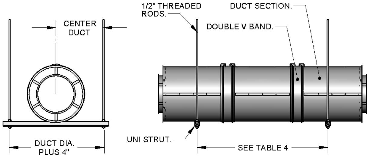
Fig. 9 – Horizontal Support Details
