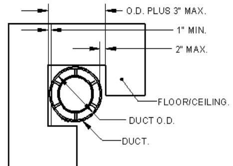
Fig. 11 – Annular Distance
