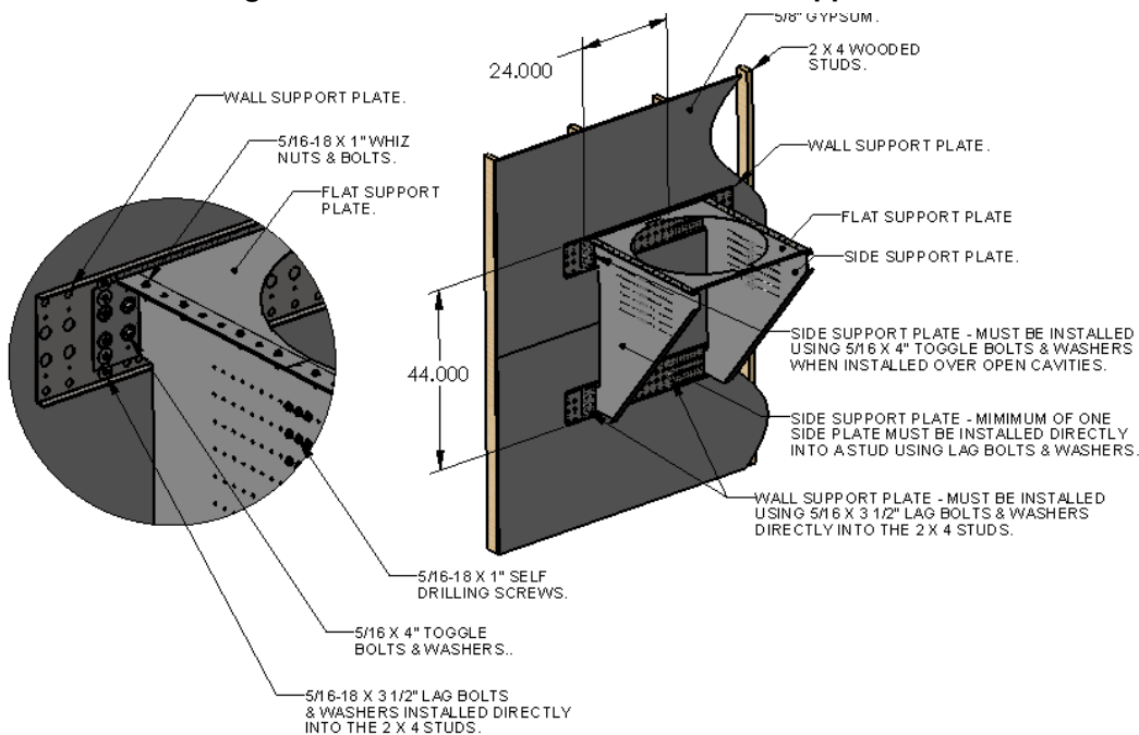
Figure 10B – Wooden Stud Wall Vertical Support
