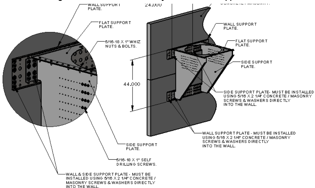
Figure 10D – Concrete/Masonry Wall Vertical Support
