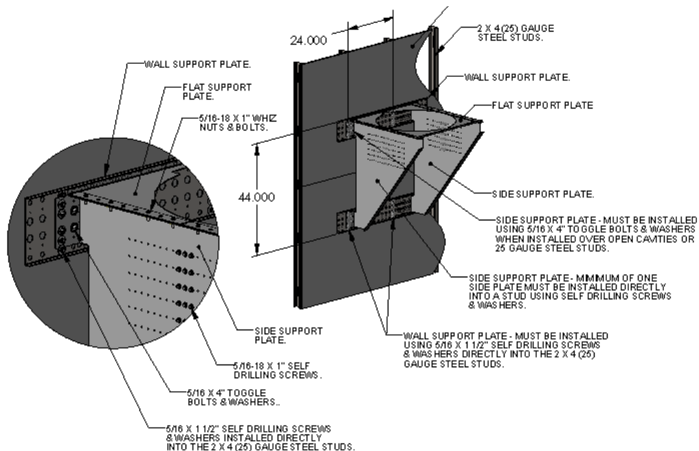
Figure 10C – Steel Stud Wall Vertical Support
